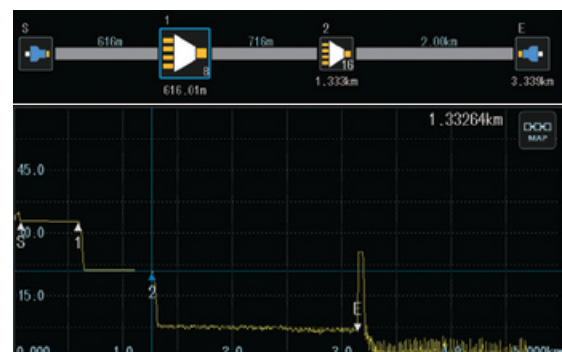
Measurement example of 128-branch splitter
